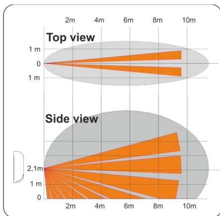
Certified diagram of detection
